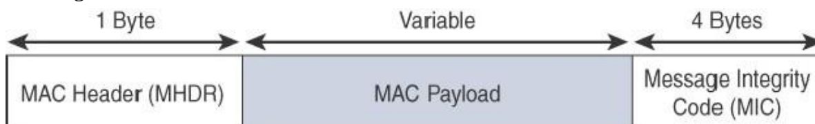
Figure 2.9 High-Level LoRaWAN MAC Frame Format
