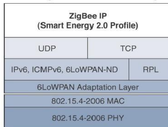
Figure : ZigBee IP protocol stack
