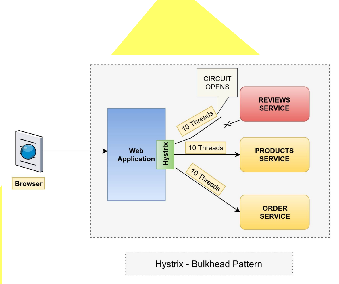
Bulkhead Design Pattern using hystrix
