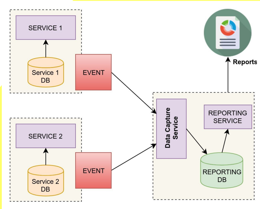
Right approach to implement Reporting Service Model
