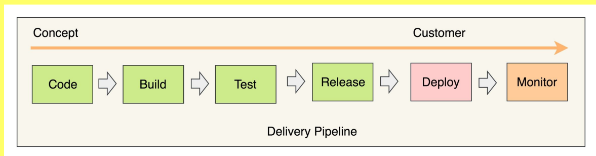
Continuous Delivery Pipeline
