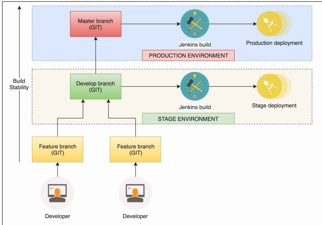
Git workflow and deployment pipeline
