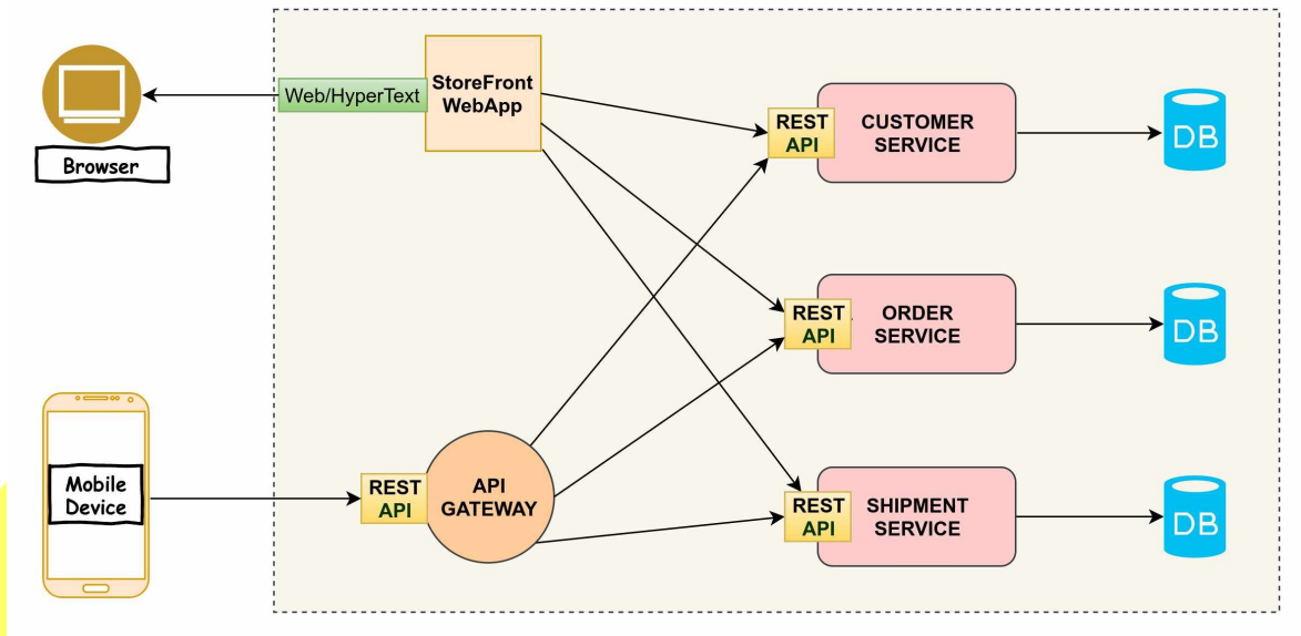
A Typical Architecture Microservices using Spring Cloud
