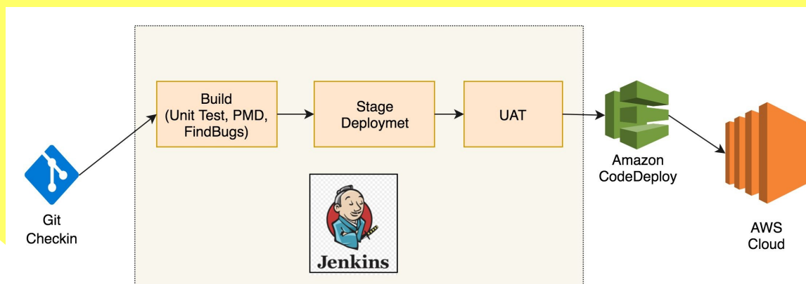
AWS Code Deploy pipeline
