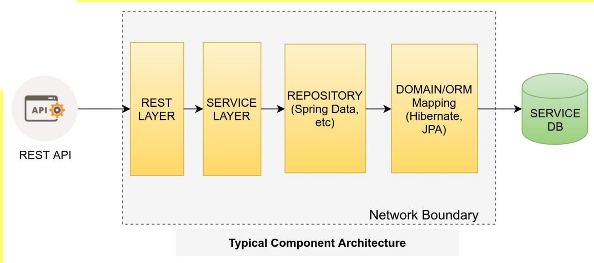
Different Layers in a Single Microservice
