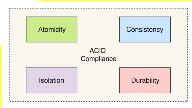
ACID compliance
