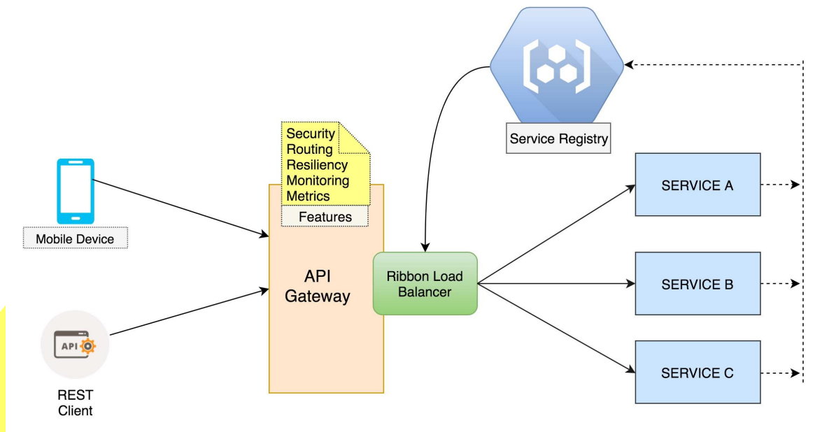
API Gateway
