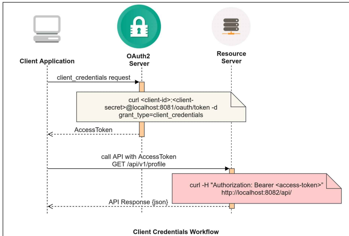
Client Credentials Sequence Diagram
