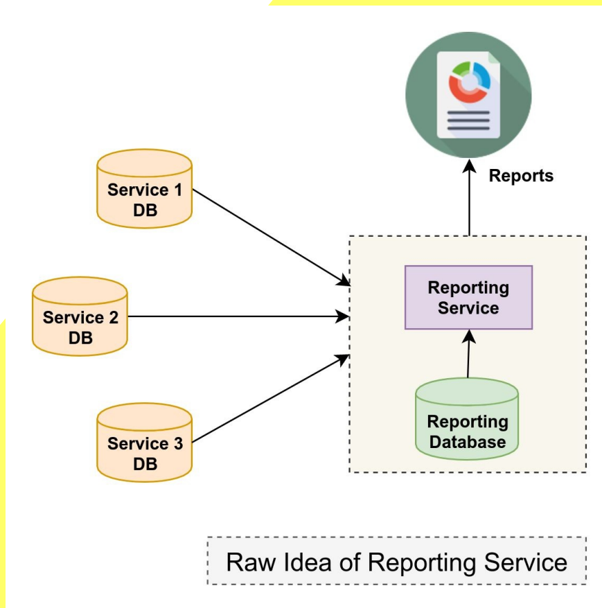
Reporting microservice - raw idea
