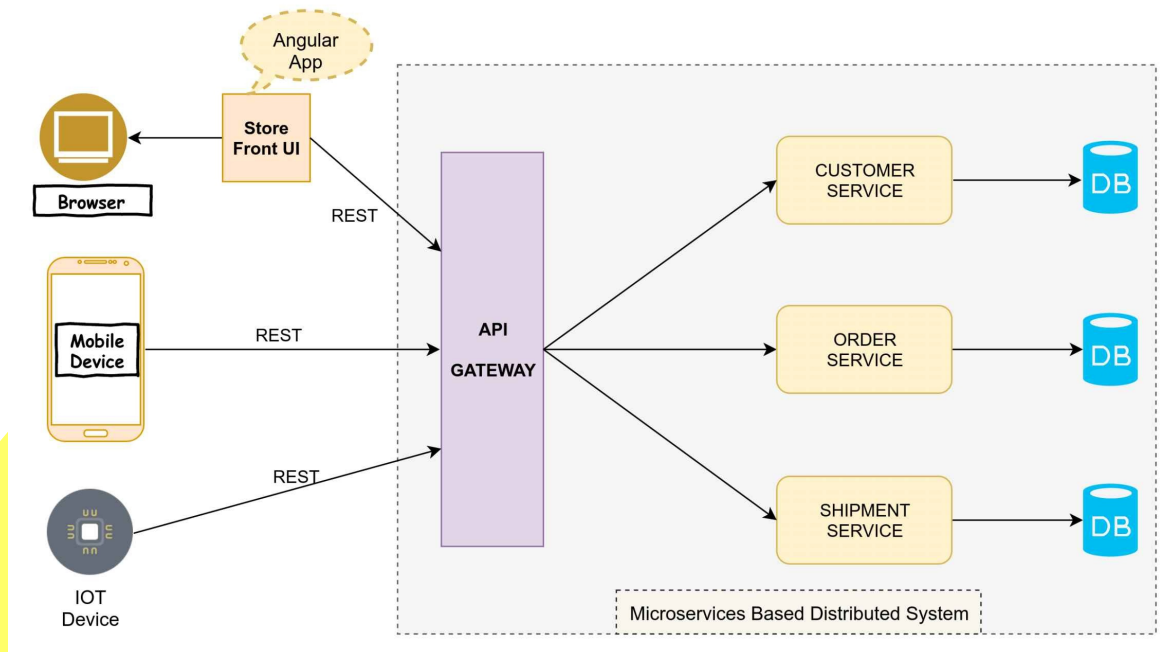
Typical Microservices Architecture Spring Boot
