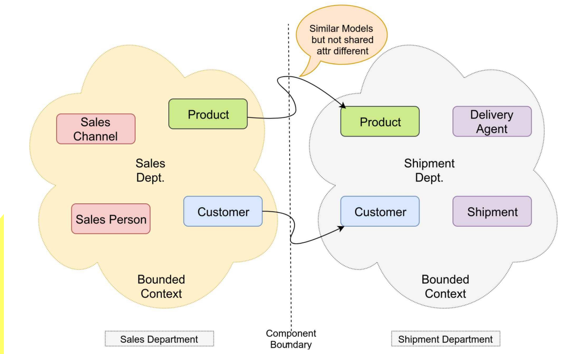
Bounded Context for sales and shipment departments of an enterprise
