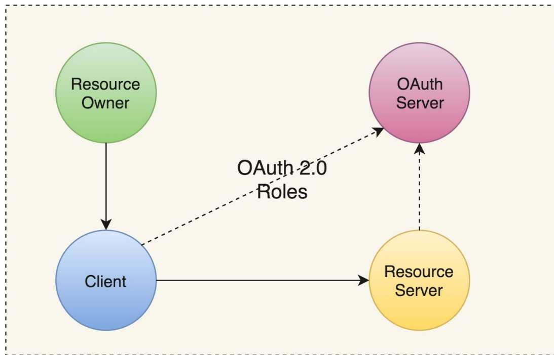
Four different roles in OAuth 2.0 protocol
